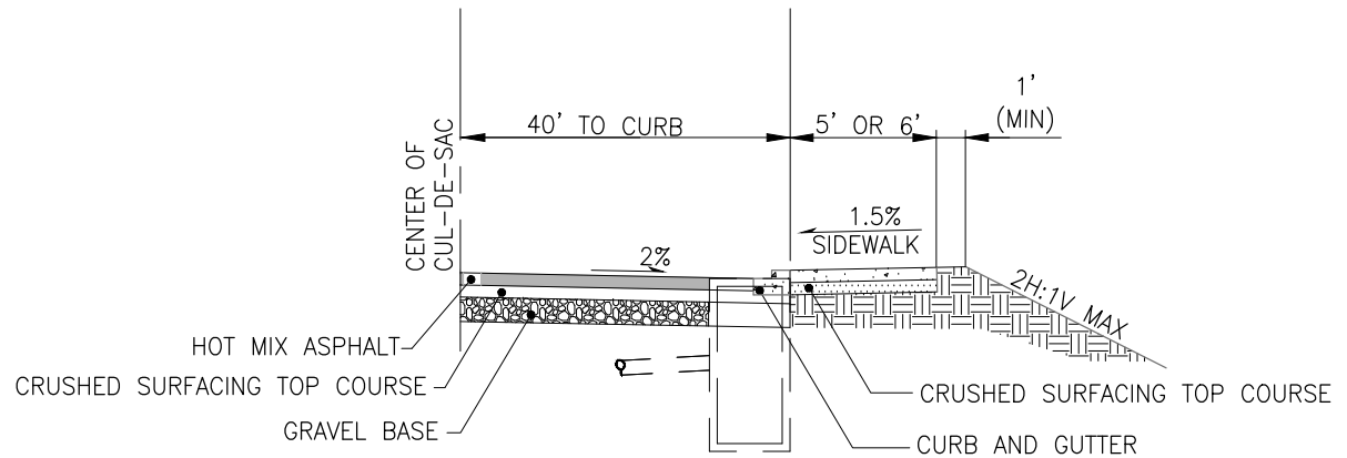
TYPICAL SECTION A-A REFER TO STANDARD DRAWING DM.A5.1 FOR PAVEMENT SECTION DETAILS.
